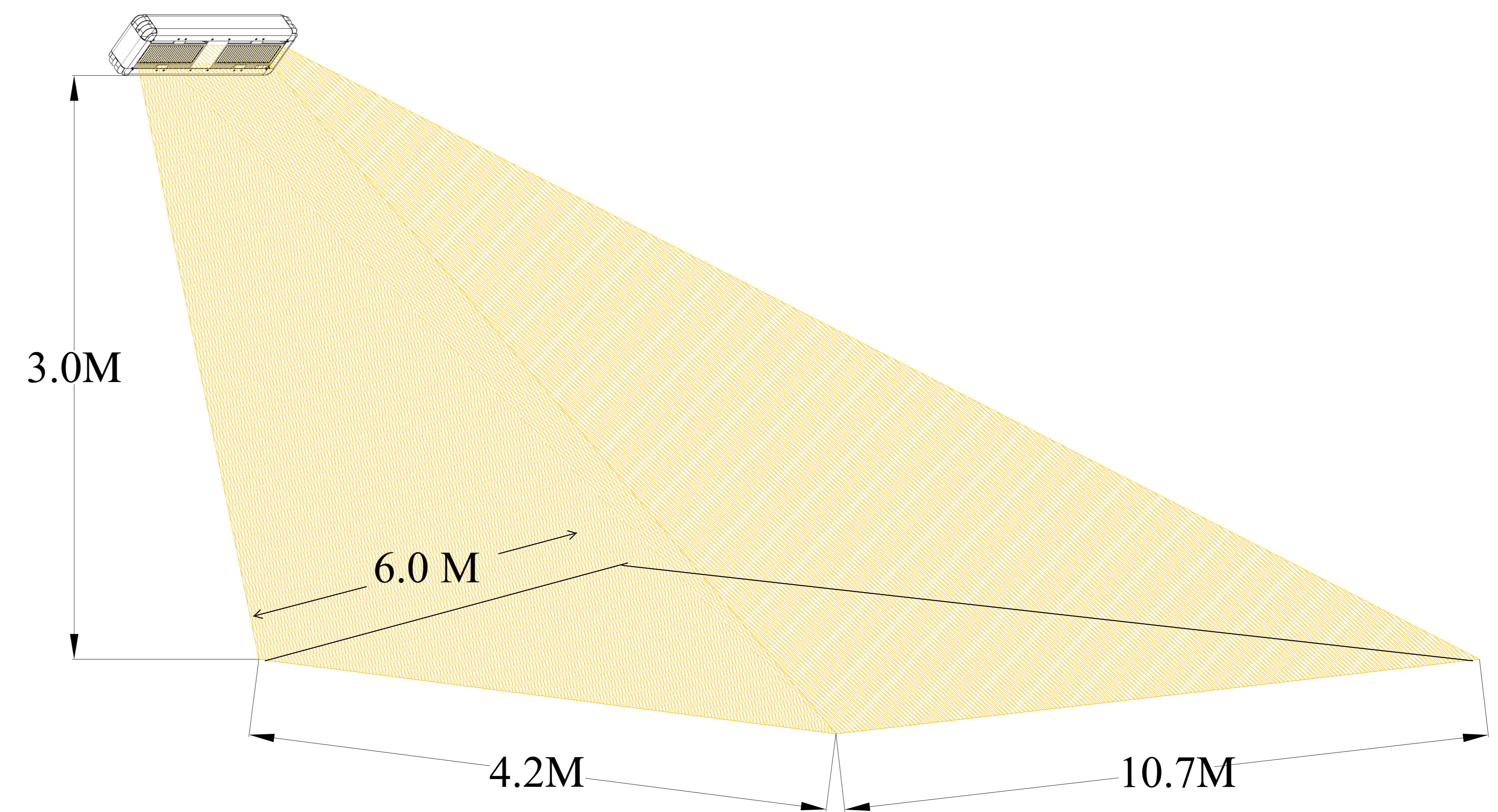
Model : Shadow Industrial 903670 - 3 or 4kW Infrared Heater Heat coverage diagram for wall installation
