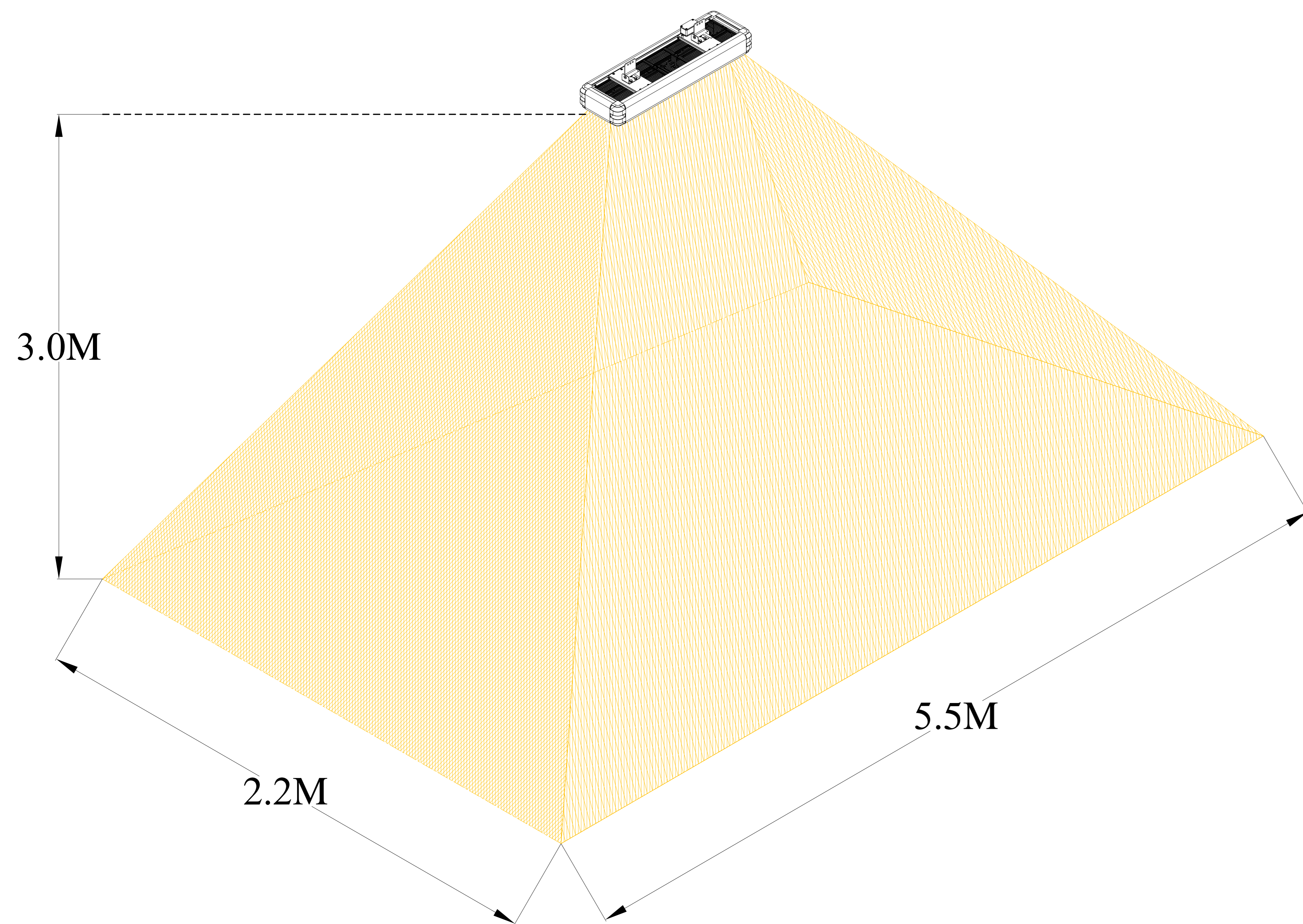
Model : Shadow Industrial 903670 - 3 or 4kW Infrared Heater Heat coverage diagram for ceiling installation
